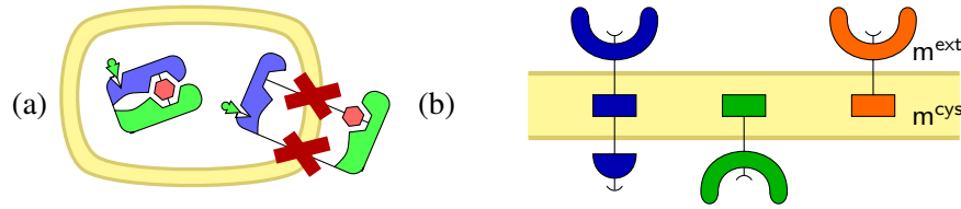
Figure 6: (a) Solution not respecting membrane impermeability; (b) Trans-membrane proteins with different orientations.
