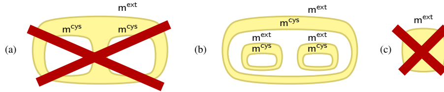
Figure 7: (a) Wrong nesting. (b) Good nesting. (c) Micelle.
