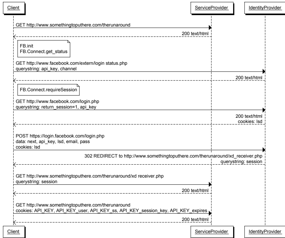
Fig. 1. Message sequence chart of the authentication flow
